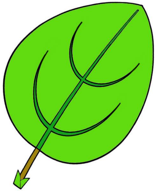
leaf
