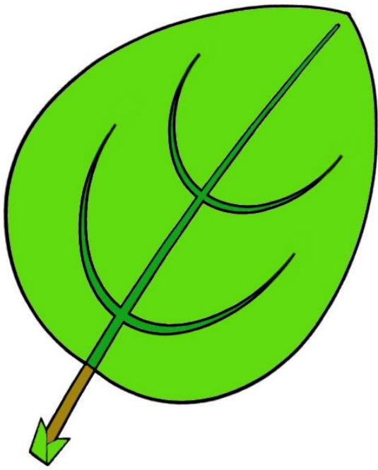
leaf
